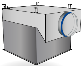
With a raised mounting base for filter depths up to 292 mm
